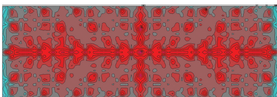
Simulated coverage of STH Arrays frequency summed at 500 to 1250 Hz
