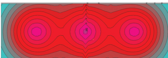
Simulated coverage of HPSA Omni frequency summed at 500 to 1250 Hz
